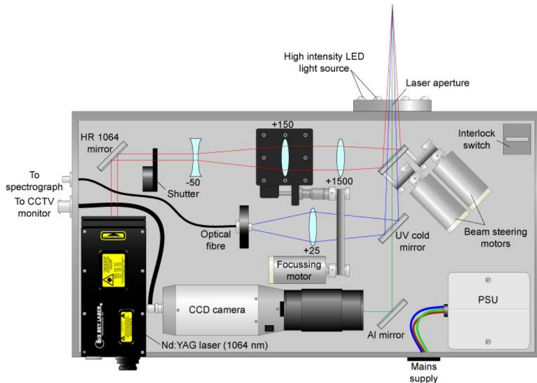
Schematic of optical arrangement
