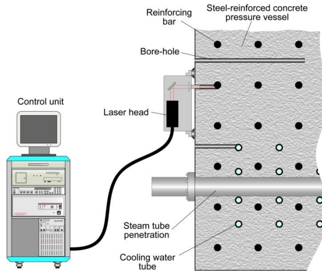
Schematic of ST-LIBS instrument deployed on reactor pressure vessel wall
