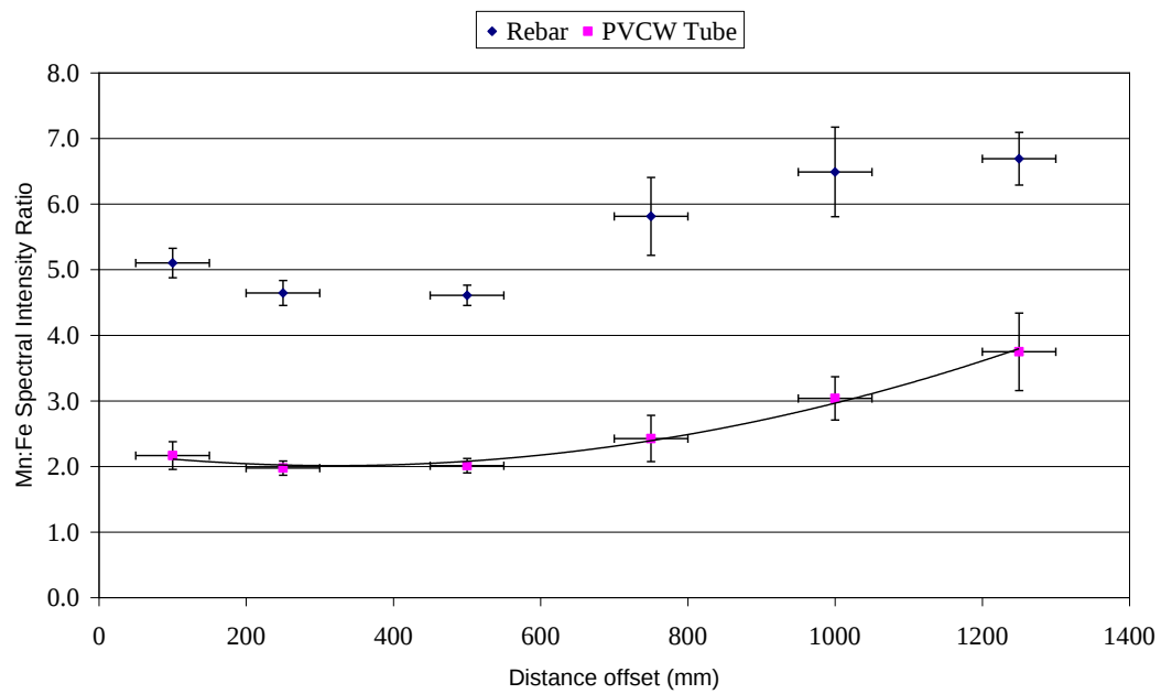
Mn:Fe spectral intensity ratios for Rebar and PVCW tubes at a range of distances between the ST-LIBS instrument and the samples
